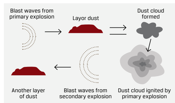
Figure 2 Primary and Secondary Dust Explosions [17]
